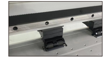
Two-foot pinch rollers
